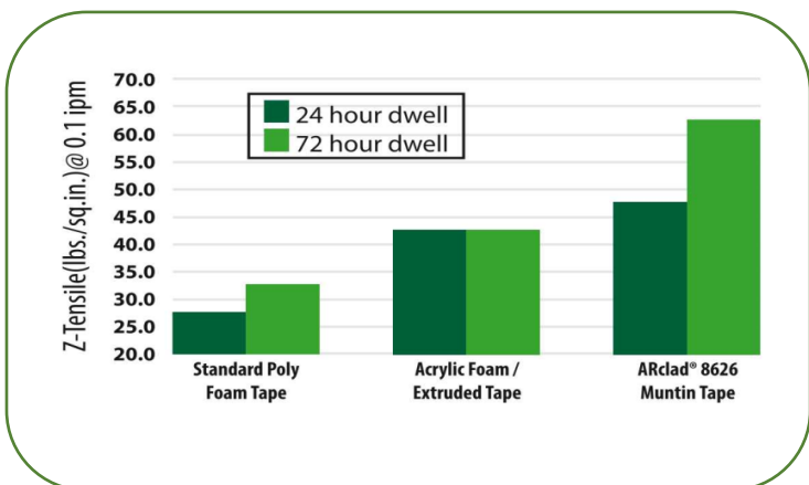
Z-Tensile Strength of Window Grille Assembly Tape
