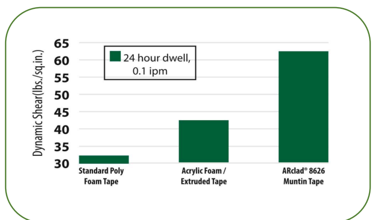
Dynamic Shear Strength of Window Grill Assembly Tape
